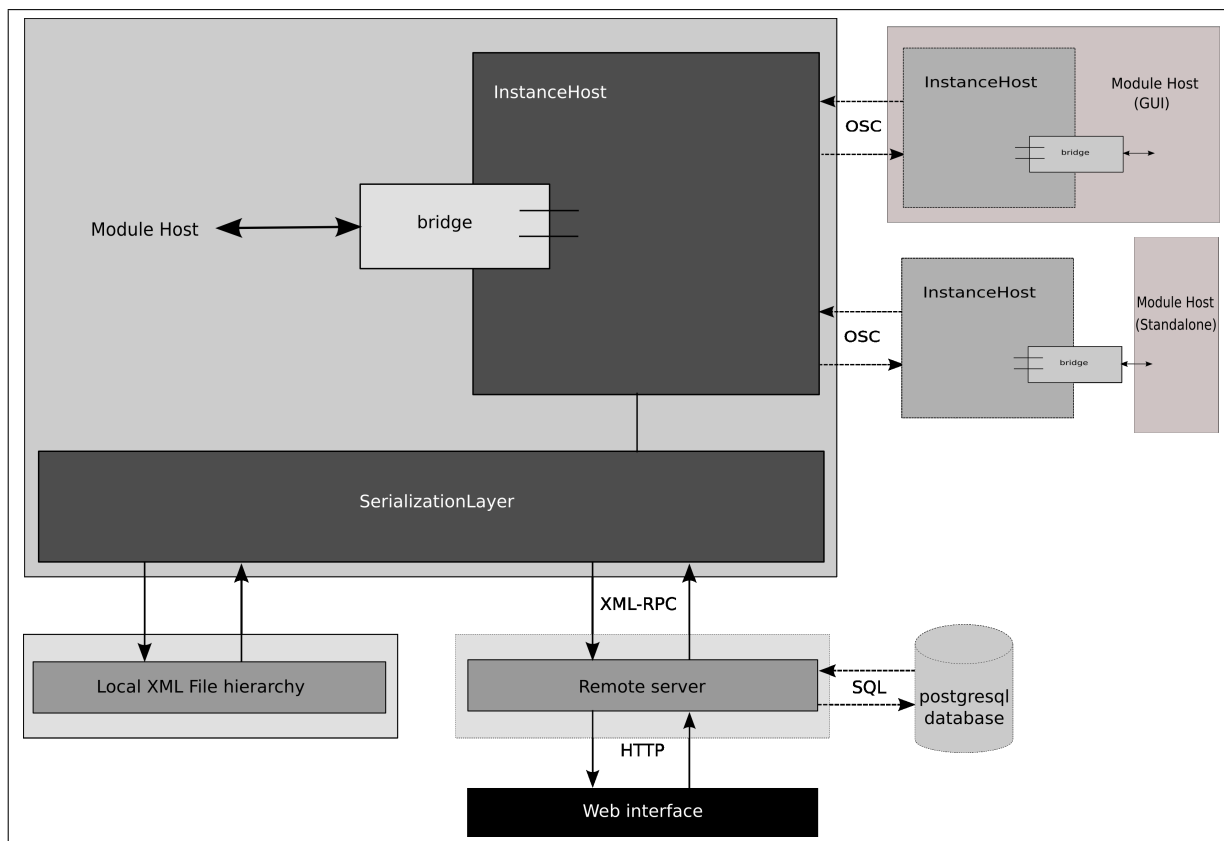
Figure 1. A model of the parts constituting libIntegra and how the library interfaces with other parts of the system.
